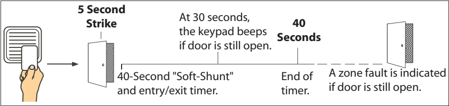
Figure 7: Door Strike Relay Operation Time Line
