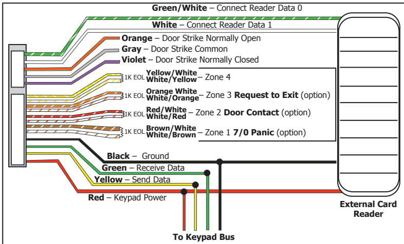
Figure 2: 12 VDC Reader Wiring for 7073/7073A and 793 Keypads
